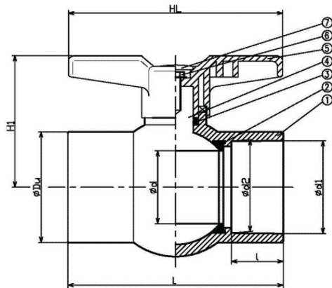
Compact Ball Valve
